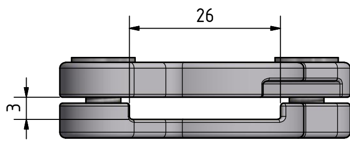
VIEW 3 SCALE 1.5 : 1
