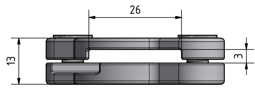
VIEW 1 SCALE 1.5 : 1
